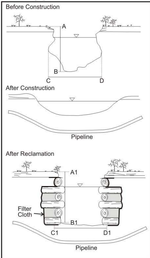
A. Overhanging Banks - Crib Wall
