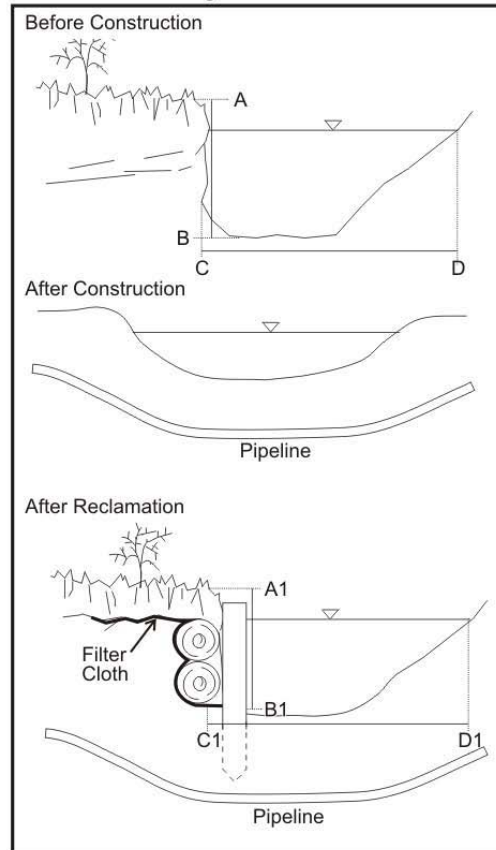
B. Vertical Banks - Log Wall
